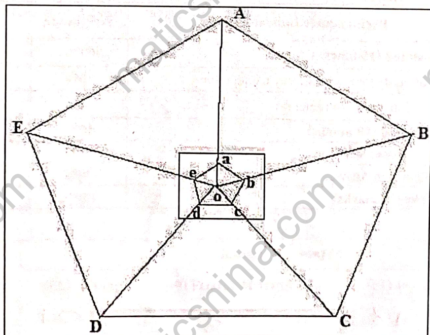
Figure No. 18.1 Radiation method of Plane Table Survey
